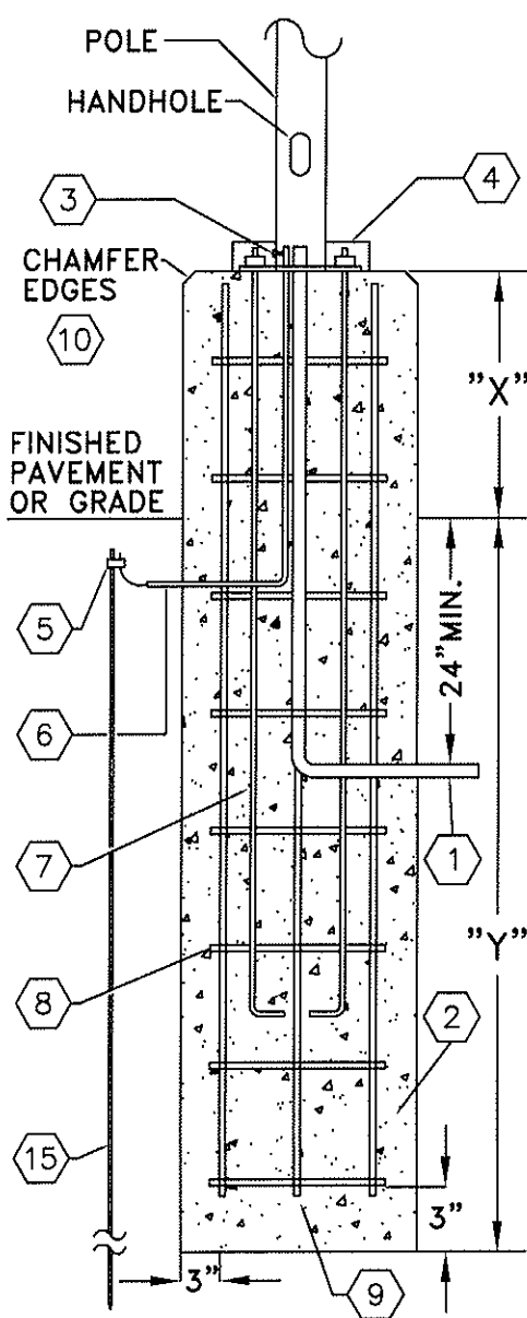
SECTION VIEW
